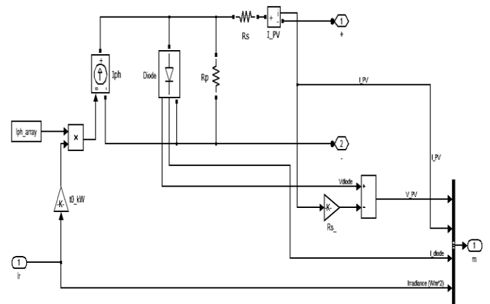
Figure 6. PV Array Structure in Matlab-Simulink.
