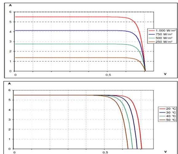
Figure 1. Nonlinearity characteristics of PV solar cell due to effect of solar irradiation and temperature [8]
