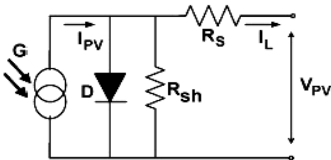
Figure 2. Equivalent Circuit diagram of the PV model [9]
