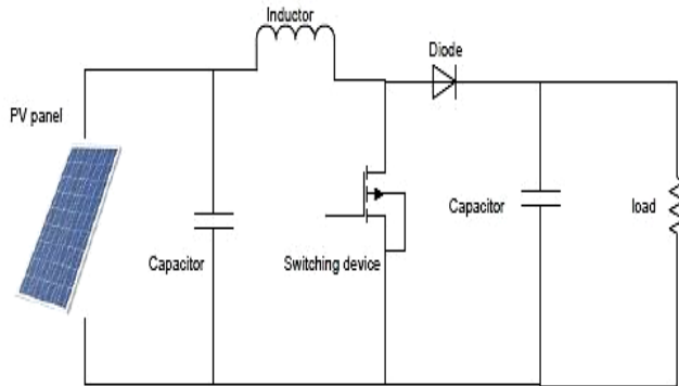
Figure 3. PV panel connected with dc-dc boost converter [14].
