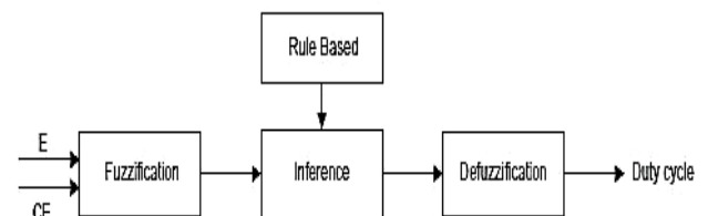
Figure 4. Block diagram of FLC method [5].
